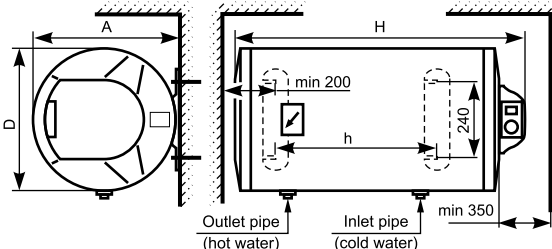
Fig. 4 Water heaters 72265X, 72270X and 72266X – 80, 100 and 120 L.
