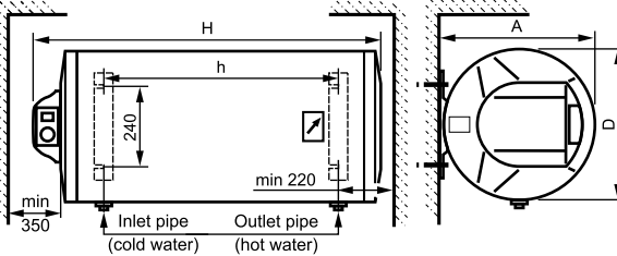
Fig. 4 Water heaters 72265X, 72270X and 72266X – 80, 100 and 120 L.
